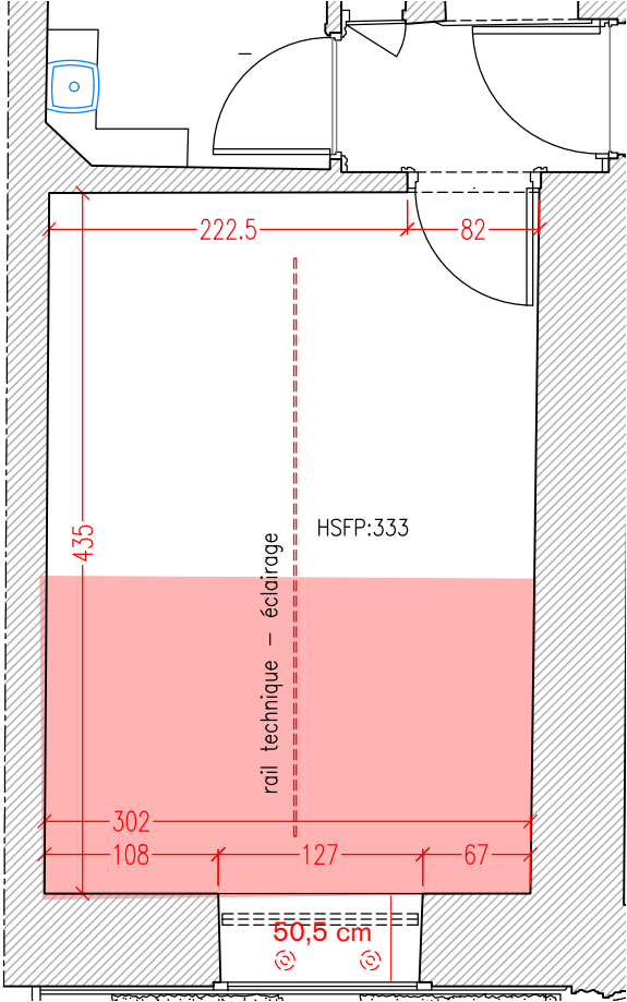
window depth with store open: 50,5 cm with store closed: 44 cm
