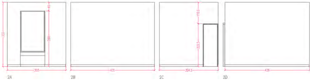
window depth with store open: 50,5 cm with store closed: 44 cm
